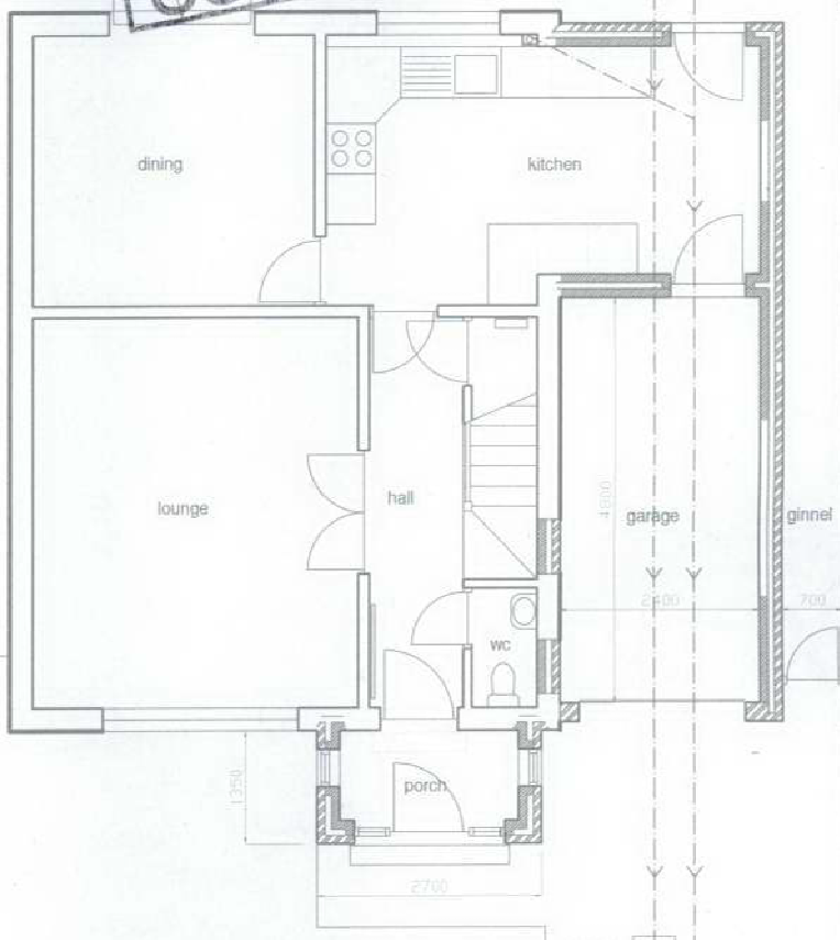
Ground Floor Plan ( proposed )
